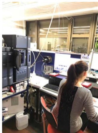
UPLC-MS analytics
